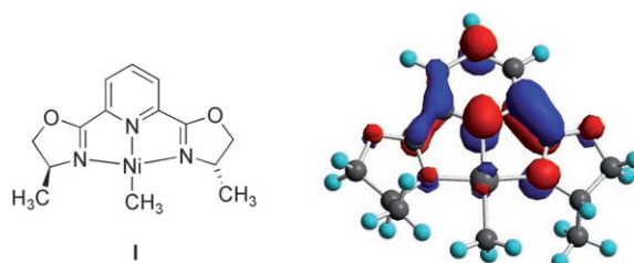
Figure 1. Optimized structure of complex I showing the ligand-centered singly occupied molecular orbital.
