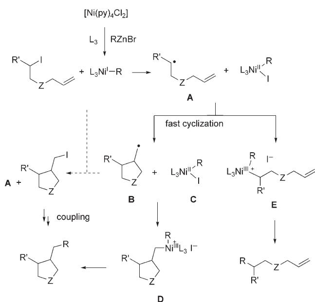
Scheme 6. Possible mechanistic pathways for the nickel-catalyzed cyclization/coupling reaction.
