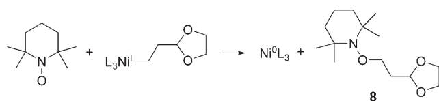
Scheme 4. Possible mechanism for the formation of 8 .
