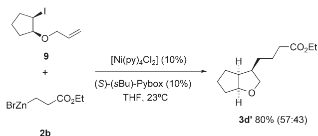
Scheme 3. Reaction of the cis stereoisomer of 1d gives the same isomeric ratio.
