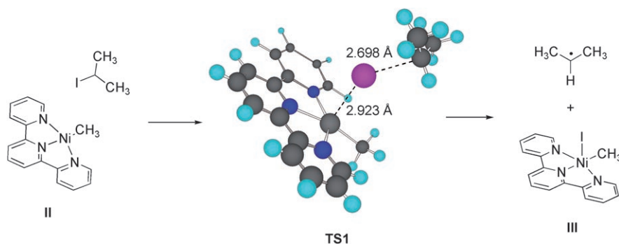
Scheme 5. Calculated transition state (DFT level) for the reaction of alkyl–nickel(I) complex with 2-iodopropane.
