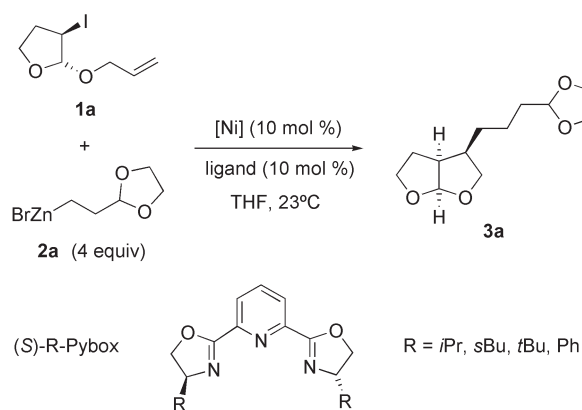
Scheme 1. Ni-catalyzed cyclization/cross-coupling reaction.
