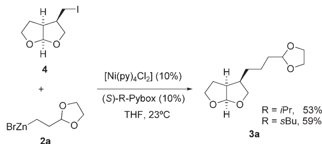
Scheme 2. Cross-coupling of 4 affords the coupling product 3a .
